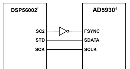
Figure 39. DSP56002 to AD5930 Interface
